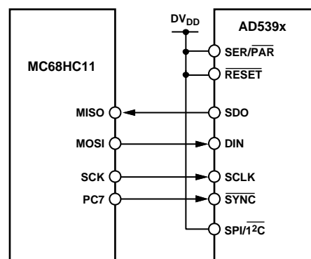
Figure 36. AD539x-MC68HC11 Interface
