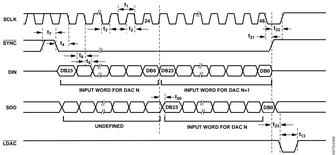
Figure 2. Serial Interface Timing Diagram (Daisy-Chain Mode)
