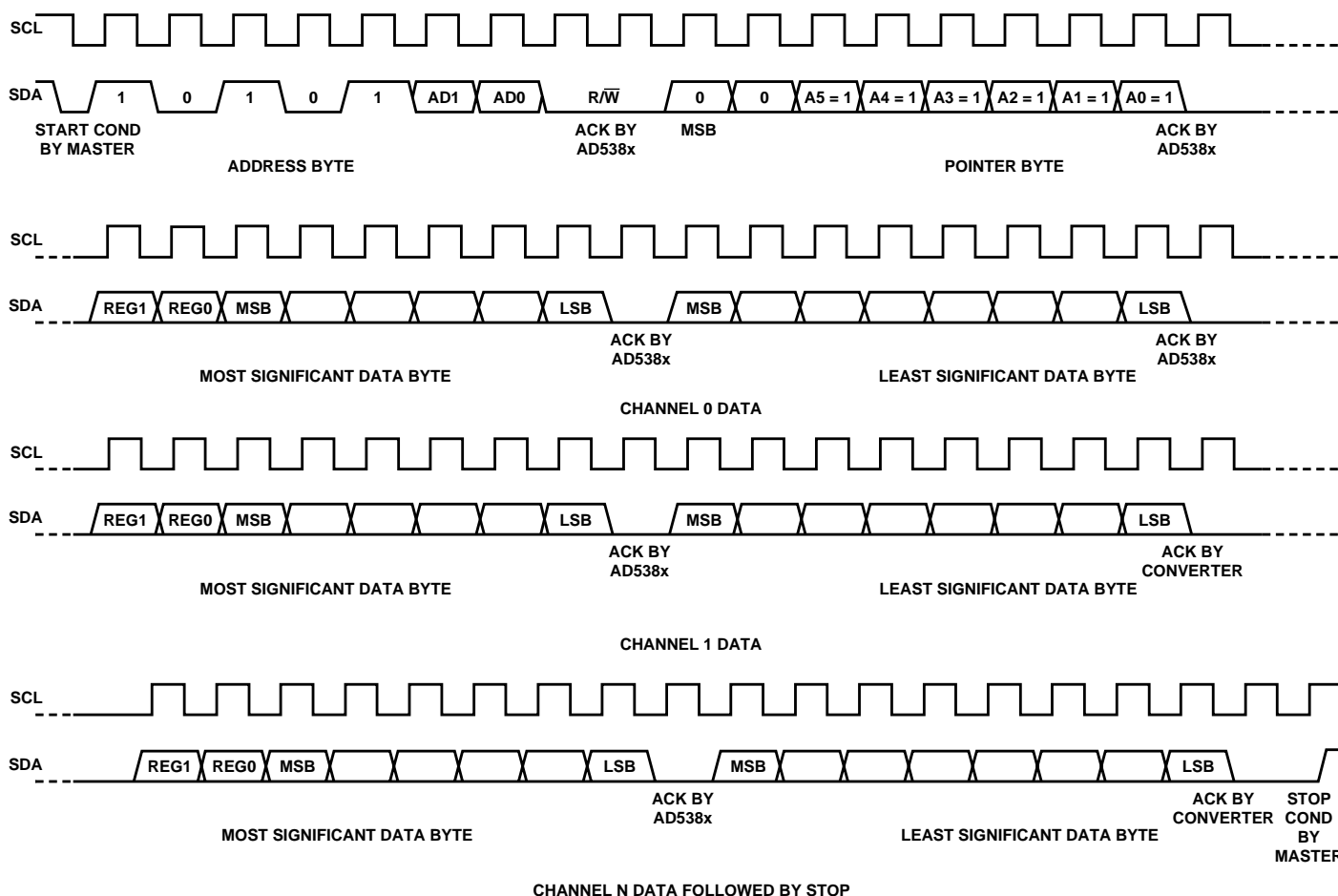
Figure 31. 2-Byte, 1²C Write Operation
