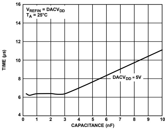
Figure 23. DAC Settling Time vs. Capacitive Load
