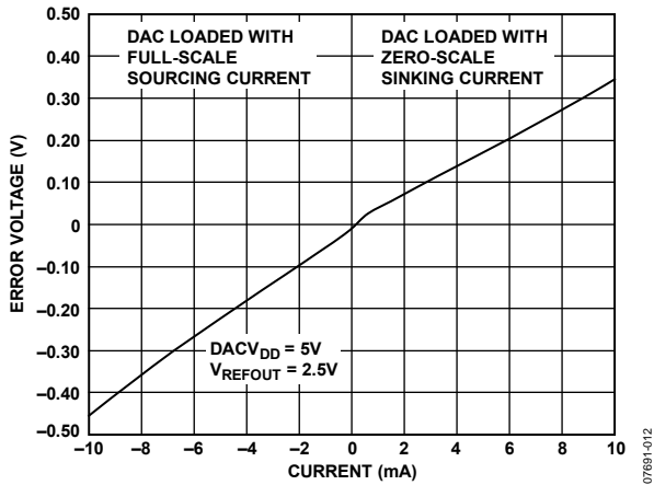
Figure 12. DAC Headroom at Rails vs. Source and Sink
