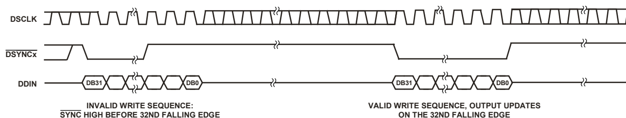
Figure 63. SYNC Interrupt Facility
