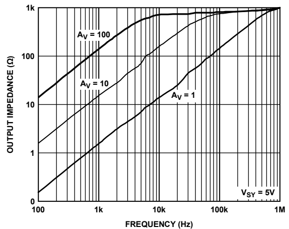
Figure 42. Amplifier Closed-Loop Output Impedance vs. Frequency
