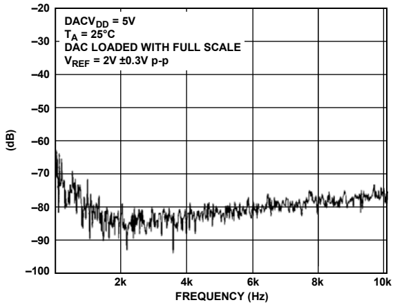
Figure 22. DAC Total Harmonic Distortion
