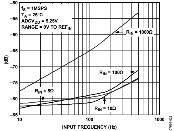
Figure 28. ADC THD vs. Input Frequency for Various Analog Source Impedances
