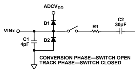
Figure 56. Equivalent Analog Input Circuit
