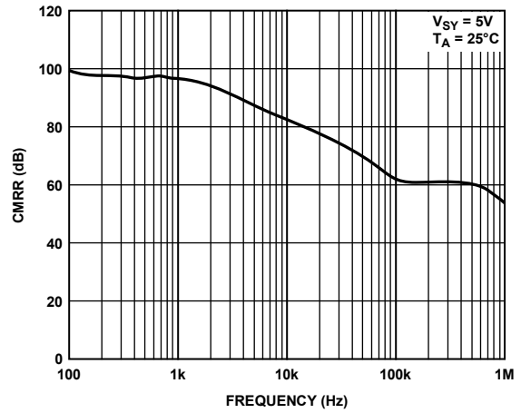
Figure 40. Amplifier CMRR vs. Frequency
