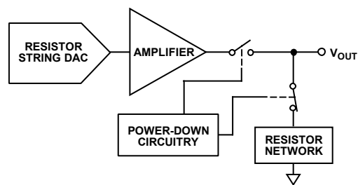
Figure 62. Output Stage During Power-Down
