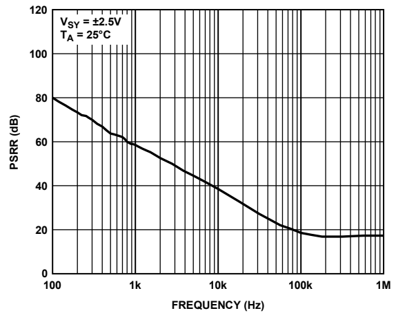
Figure 41. Amplifier PSRR vs. Frequency
