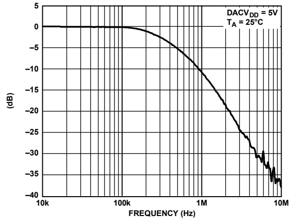
Figure 24. DAC Multiplying Bandwidth
