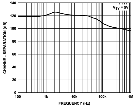
Figure 51. Amplifier Channel Separation
