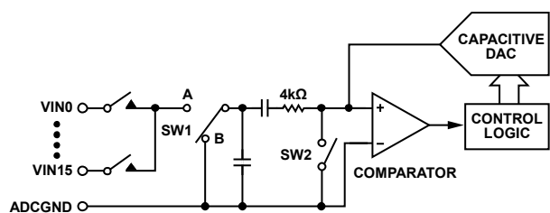
Figure 55. ADC Conversion Phase
