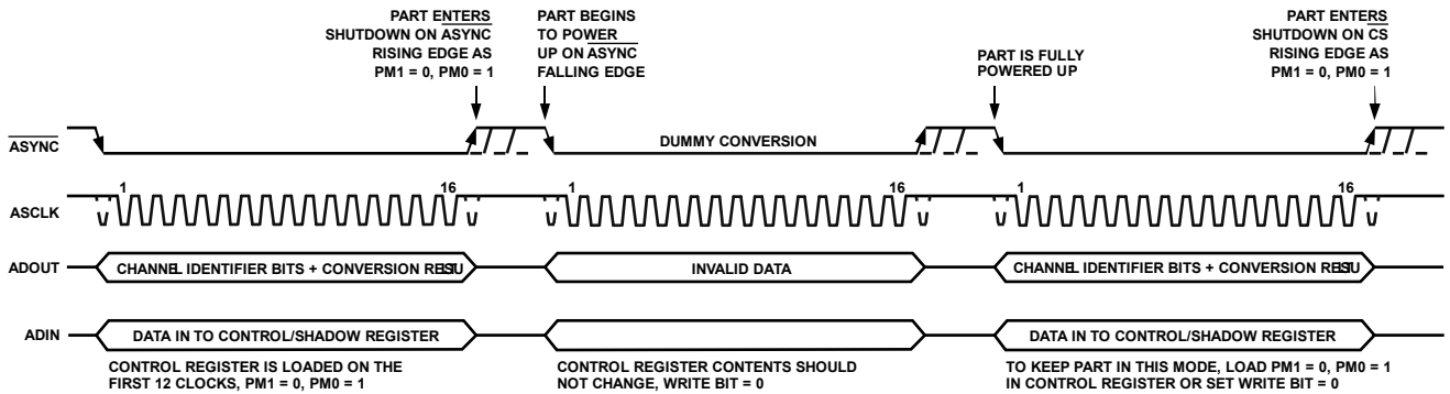
Figure 66. Autoshtutdown Mode Operation
