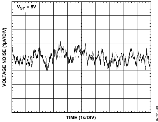
Figure 49. Amplifier 0.1 Hz to 10 Hz Input Voltage Noise
