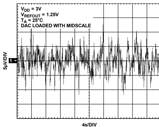
Figure 47. 0.1 Hz to 10 Hz Output Noise Plot, 1.25 V Internal Reference
