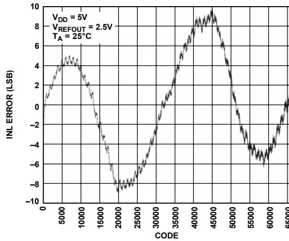
Figure 12. AD5667R INL, 2.5 V Internal Reference
