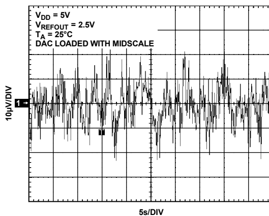
Figure 46. 0.1 Hz to 10 Hz Output Noise Plot, 2.5 V Internal Reference
