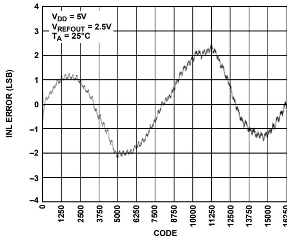
Figure 13. AD5647R INL, 2.5 V Internal Reference
