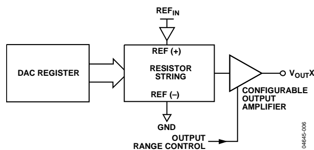
Figure 42. DAC Architecture Block Diagram
