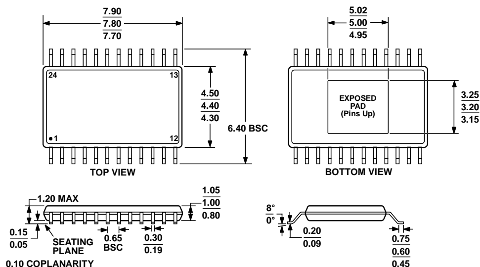
Figure 49. 24-Lead Thin Shrink Small Outline Package, Exposed Pad [TSSOP_EP] (RE-24) Dimensions shown in millimeters
