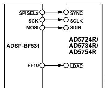
Figure 48. AD5724R/AD5734R/AD5754R to Blackfin Interface
