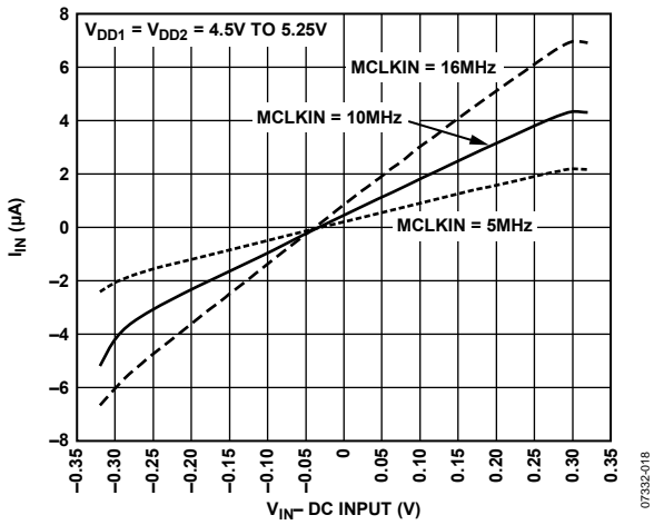
Figure 18. I_{IN} vs. V_{IN} -DC Input
