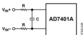
Figure 25. Differential Input RC Network
