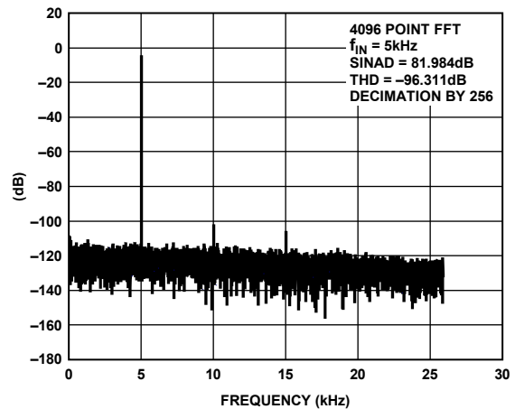
Figure 8. Typical FFT ( \pm 200 mV Range)
