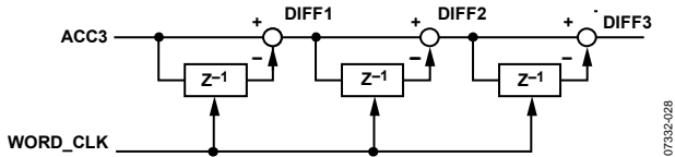
Figure 28. Differentiator
