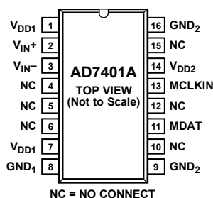
Figure 5. Pin Configuration
