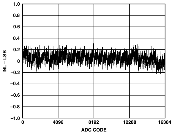
TPC 2. Typical INL
