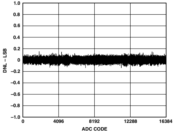
TPC 1. Typical DNL
