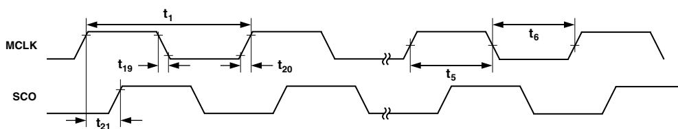
Figure 15. Serial Clock Timing
