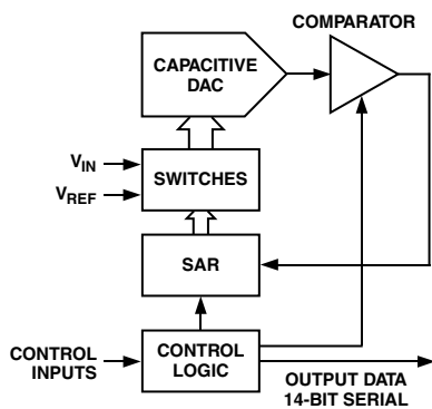
Figure 3. Simplified Block Diagram
