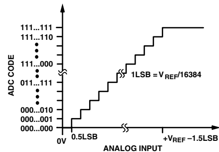
Figure 6. Transfer Characteristic
