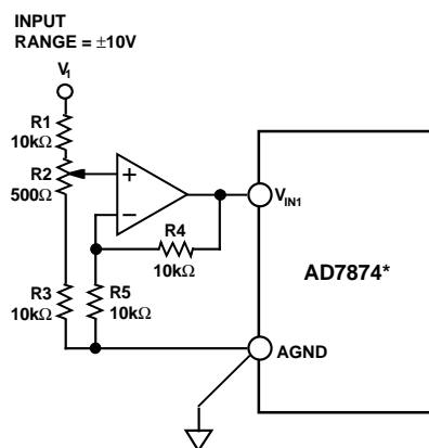
Figure 6. AD7874 Full-Scale Adjust Circuit
