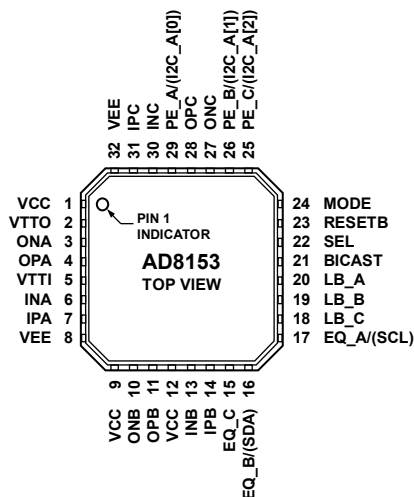
Figure 3. Pin Configuration
