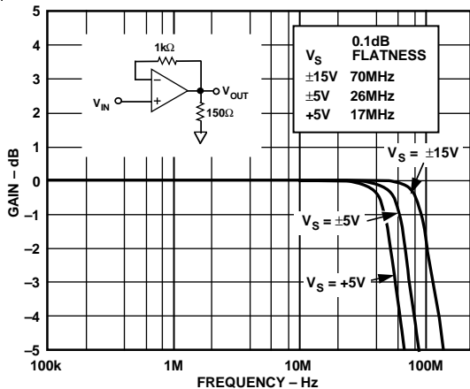
Figure 21. Closed-Loop Gain vs. Frequency, Gain = +1
