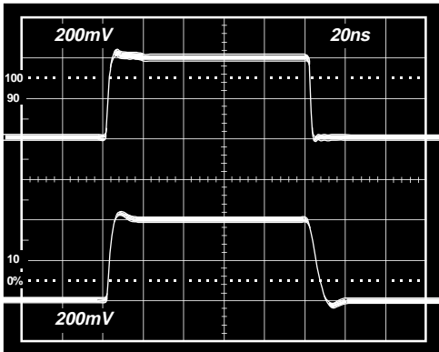
Figure 26. Noninverting Small Signal Pulse Response, R_L = 150 \Omega
