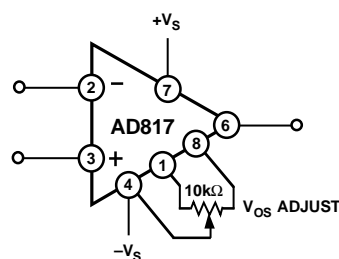
Figure 32. Offset Nulling Circuit
