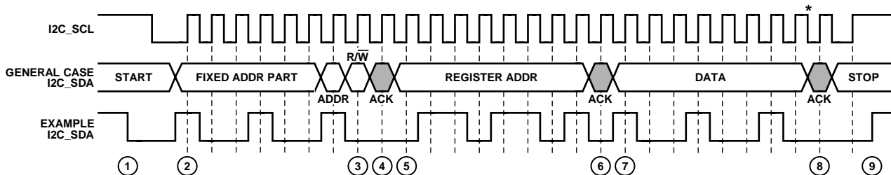
Figure 29. I 2 C Write Procedure
