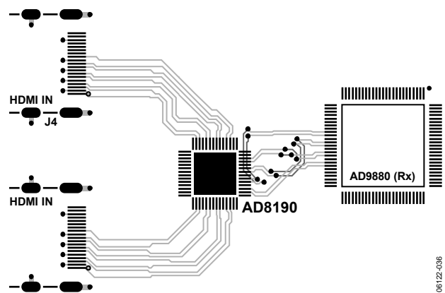
Figure 32. Layout of the TMD5 Traces for the AD8190 in an HDMI Standard Revision 1.2a Receive-Compliant Reference Design
