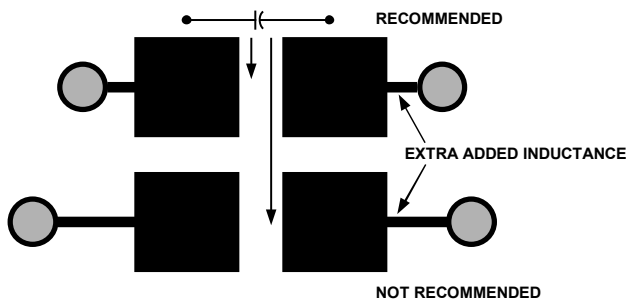
Figure 34. Recommended Pad Outline for Bypass Capacitors
