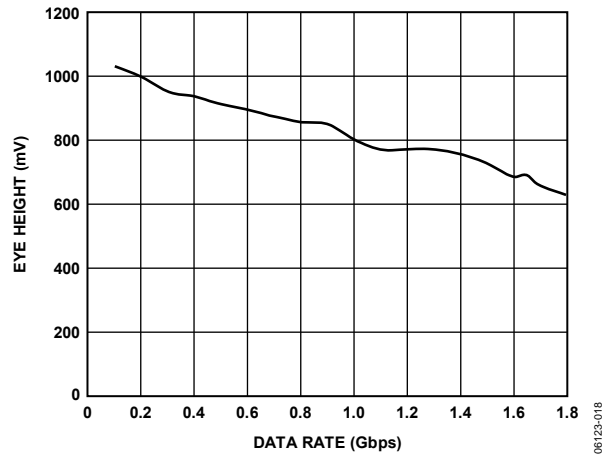
Figure 18. Eye Height vs. Data Rate
