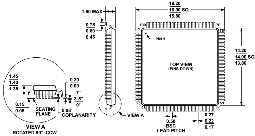
COMPLIANT TO JEDEC STANDARDS MS-026-BED Figure 35. 100-Lead Low Profile Quad Flat Package [LQFP] (ST-100) Dimensions shown in millimeters
