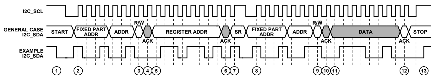
Figure 30. I 2 C Read Diagram
