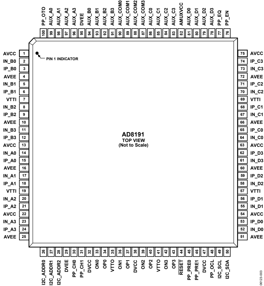
Figure 3. Pin Configuration
