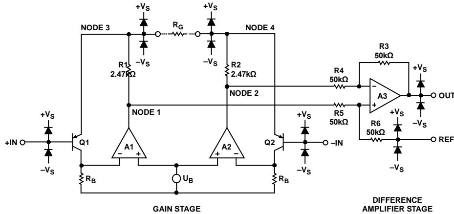
Figure 3. Simplified Schematic
