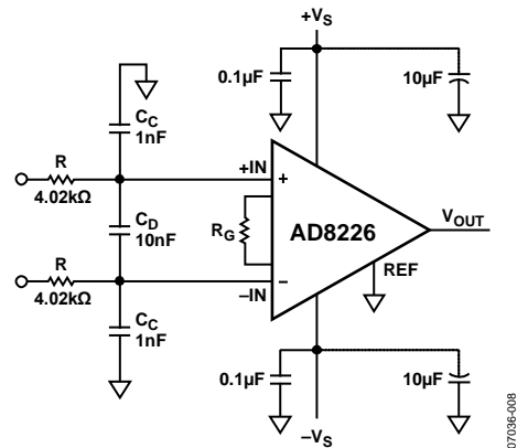
Figure 8. RFI Suppression
