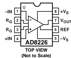
Figure 5. Pinout Diagram
