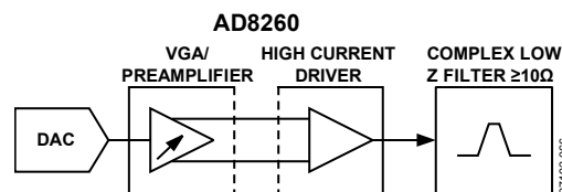
Figure 66. AD8260 Used as a VGA Driving a Low Impedance Load
