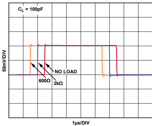
Figure 19. Small-Signal Step Response, Gain = 2
