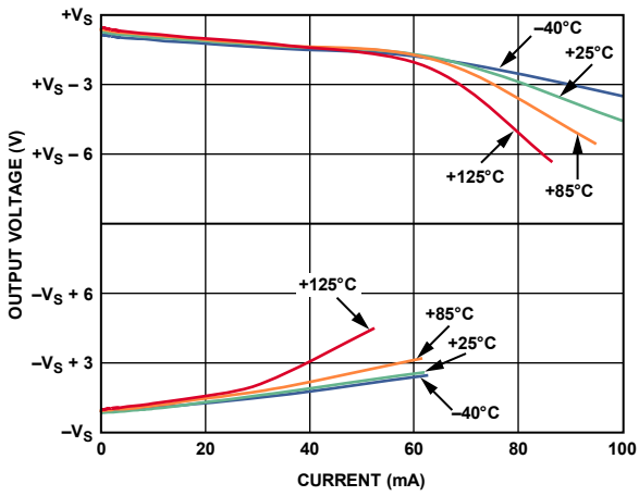
Figure 18. Output Voltage vs. I_{OUT}
