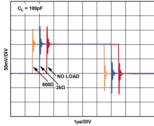
Figure 20. Small-Signal Step Response, Gain = \frac{1}{2}
