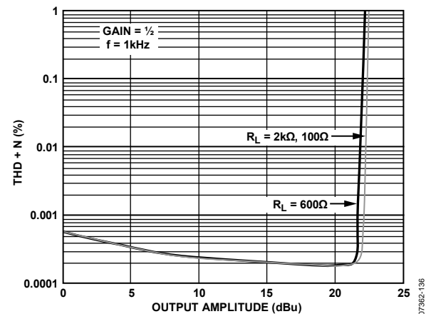
Figure 34. THD + N vs. Output Amplitude, G = \frac{1}{2}
