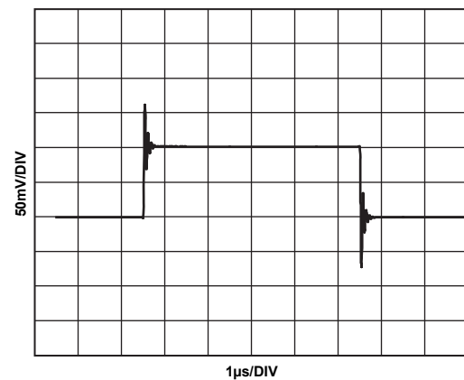
Figure 22. Small-Signal Pulse Response for 100 pF Capacitive Load, Gain = \frac{1}{2}
