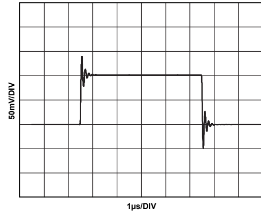
Figure 21. Small-Signal Pulse Response with 500 pF Capacitor Load, Gain = 2
