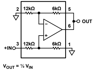
Figure 44. Noninverting Amplifier, G = \frac{1}{2}
