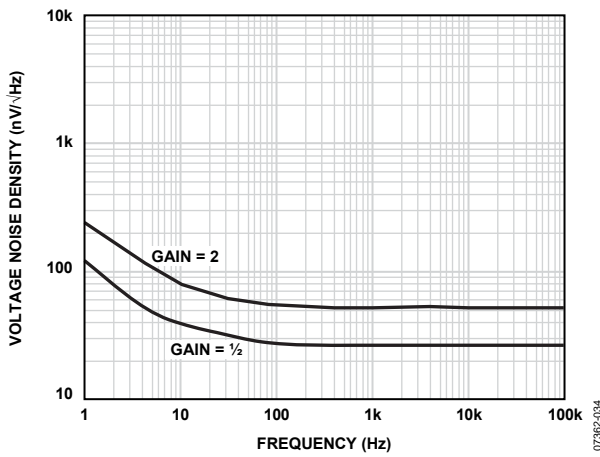
Figure 30. Voltage Noise Density vs. Frequency, Referred to Output
