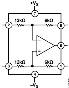
Figure 38. Functional Block Diagram
