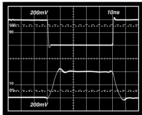
Figure 32. Inverter Small Signal Pulse Response \pm 15 V_S , C_F = 1 pF , R_L = 1500 \Omega
