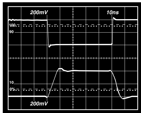
Figure 33. Inverter Small Signal Pulse Response \pm 5 V_S , C_F = 0 pF , R_L = 150 \Omega
