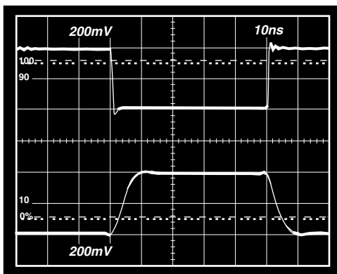
Figure 30. Inverter Small Signal Pulse Response \pm 5 V_S , C_F = 1 pF , R_L = 150 \Omega
