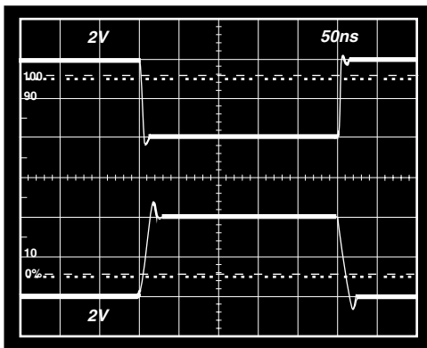
Figure 29. Inverter Large Signal Pulse Response \pm 5 V_S , C_F = 1 pF , R_L = 1 k\Omega
