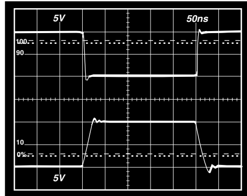
Figure 31. Inverter Large Signal Pulse Response \pm 15 V_S , C_F = 1 pF , R_L = 1 k\Omega
