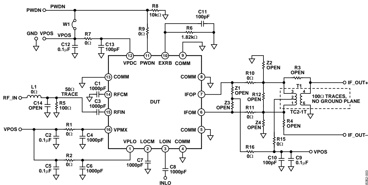
Figure 53. Evaluation Board
