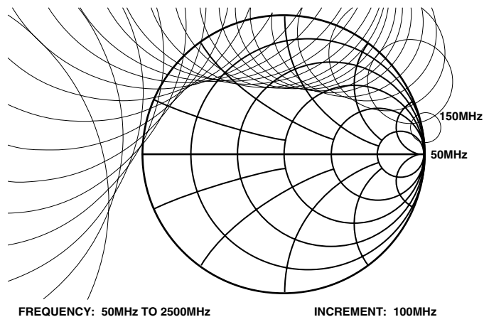
Figure 14. Common-Mode Output Stability Circles
