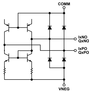
Figure 7. Output Drivers
