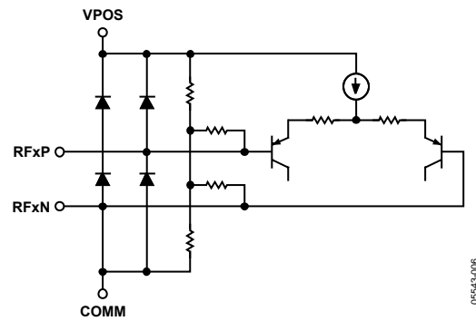
Figure 6. RF Inputs
