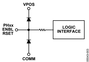
Figure 3. Logic Inputs
