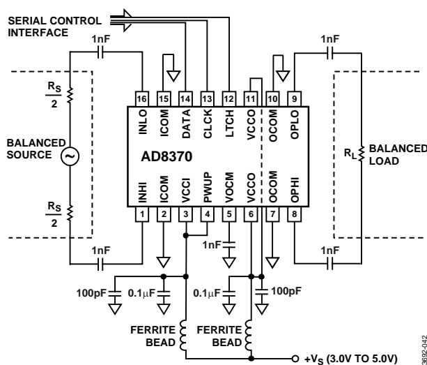
Figure 44. Basic Connections
