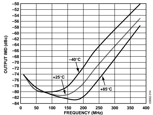
Figure 15. Two-Tone Output IMD3 vs. Frequency at Maximum Gain, R_L = 1k\Omega , V_{OUT} = 2V p-p Composite Differential
