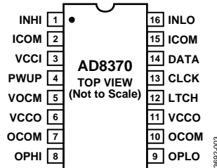
Figure 3.16-Lead TSSOP
