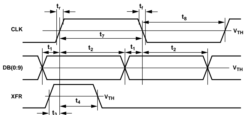
Figure 5. Input Timing
