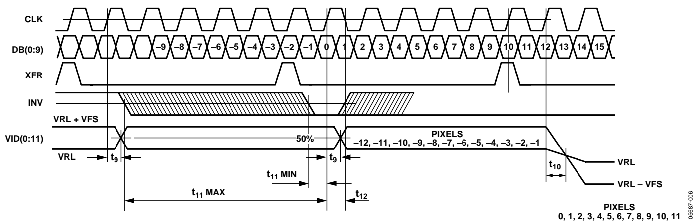
Figure 6. Output Timing (R/L LOW)
