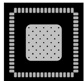
Figure 15. Solder Mask—Top Layer
