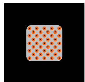
Figure 14. Land Patter—Bottom PCB Layer
