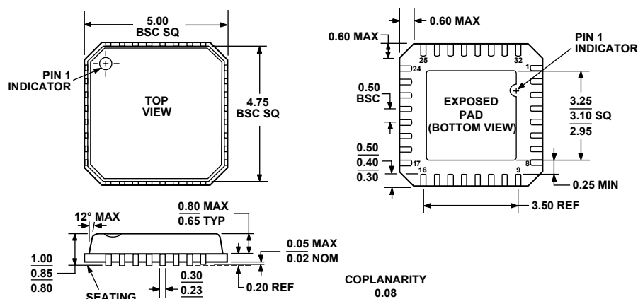
Figure 22. 32-Lead Lead Frame Chip Scale Package [LFCSP_VQ] 5 mm × 5 mm Body, Very Thin Quad (CP-32-2)
