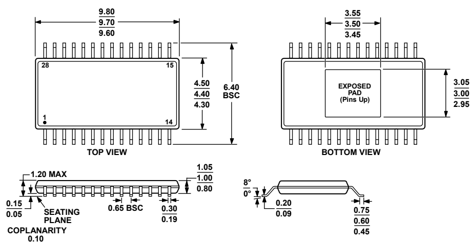
Figure 21. 28-Lead Thin Shrink Small Outline with Exposed Pad [TSSOP/EP] (RE-28-1)
