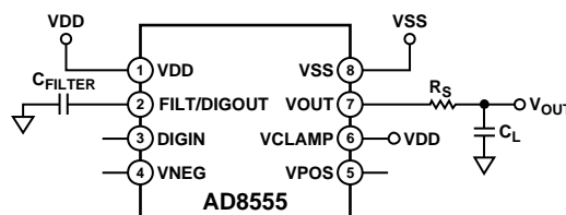
Figure 56. Test Circuit for Driving Capacitive Loads
