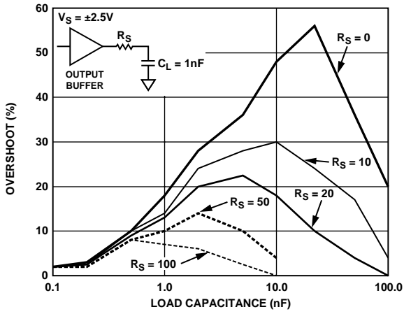
Figure 28. Output Buffer Positive Overshoot
