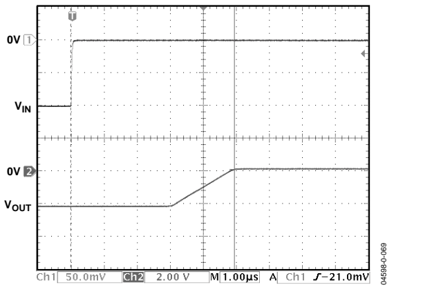
Figure 42. Negative Overload Recovery (Gain = 70)
