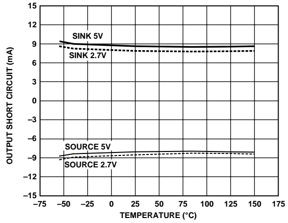
Figure 31. Output Short Circuit vs. Temperature
