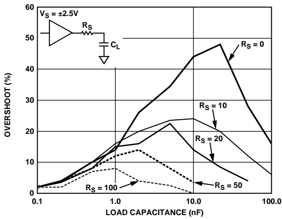
Figure 58. Negative Overshoot Graph vs. C_L
