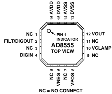
Figure 3. 16-Lead LFCSP (Not Drawn to Scale)
