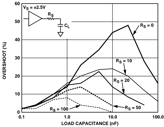
Figure 29. Output Buffer Negative Overshoot
