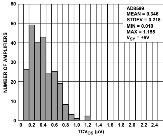
Figure 5. TCV_{OS} Distribution, -40^\circ\text{C} \leq T_A \leq +125^\circ\text{C}
