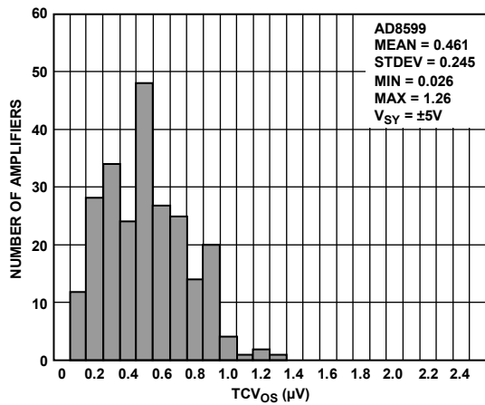
Figure 6. TCV_{OS} Distribution, -40^\circ\text{C} \leq T_A \leq +85^\circ\text{C}
