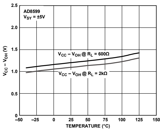
Figure 24. Output Saturation Voltage vs. Temperature
