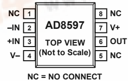
Figure 1. AD8597 8-Lead SOIC (R-8)
