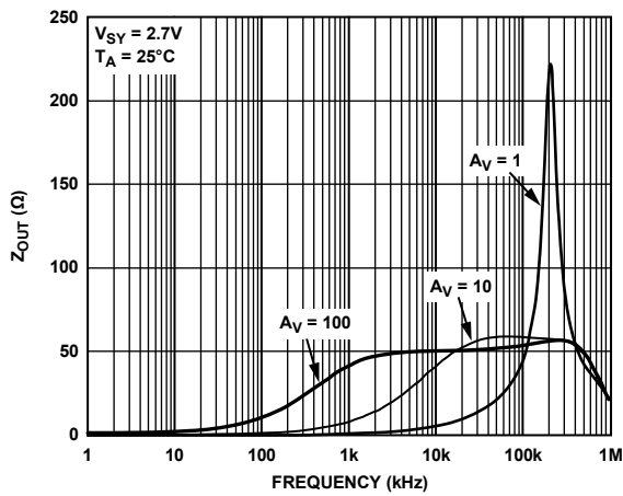
Figure 18. Z_{OUT} vs. Frequency
