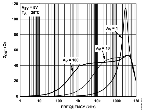
Figure 21. Z_{OUT} vs. Frequency
