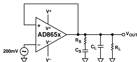
Figure 57. Snubber Network
