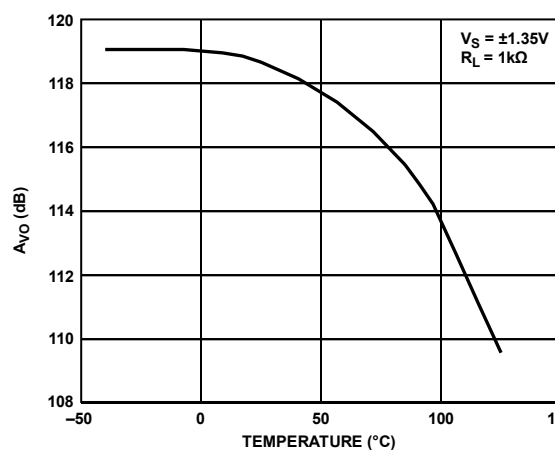
Figure 50. Open-Loop Gain vs. Temperature
