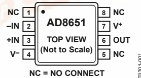
Figure 1. 8-Lead MSOP (RM-8)
