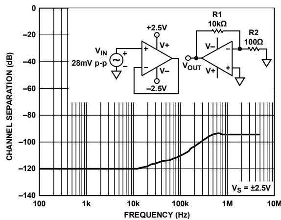
Figure 52. Channel Separation vs. Frequency.
