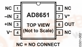
Figure 3. 8-Lead SOIC_N (R-8)
