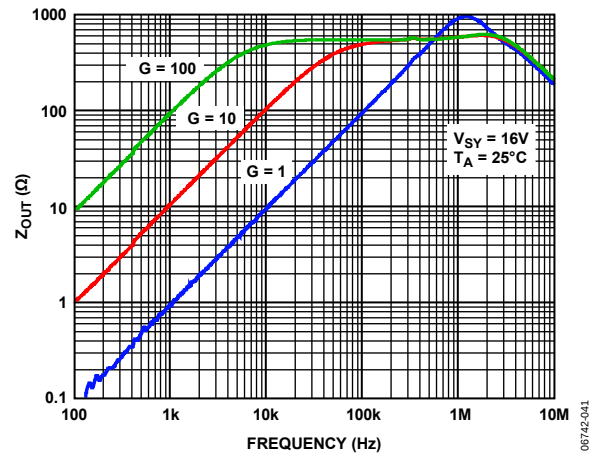
Figure 26. Closed-Loop Output Impedance vs. Frequency, V_{SV} = 16\text{ V}
