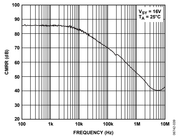
Figure 15. CMRR vs. Frequency, V_{SY} = 16\text{ V}
