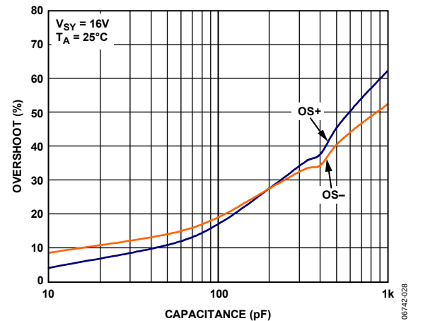
Figure 28. Small-Signal Overshoot vs. Load Capacitance, V_{SV} = 16\text{ V}
