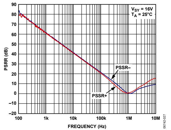
Figure 27. PSRR vs. Frequency, V_{SV} = 16\text{ V}
