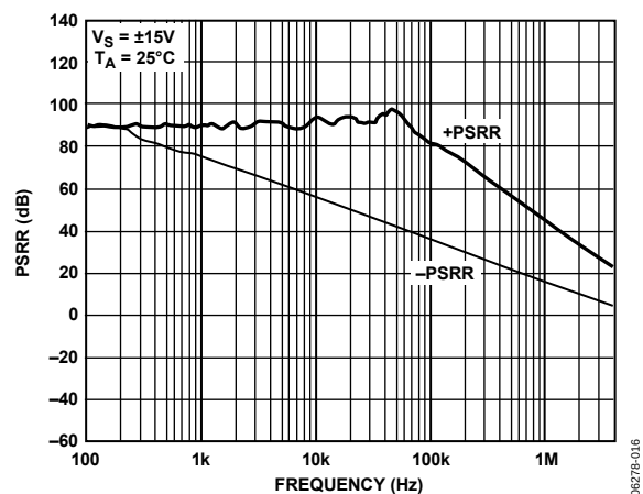
Figure 16. AD8682 PSRR vs. Frequency
