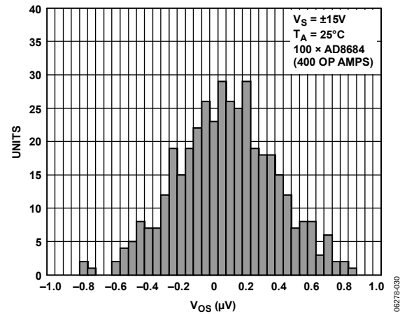
Figure 30. AD8684 V_{OS} Distribution Package
