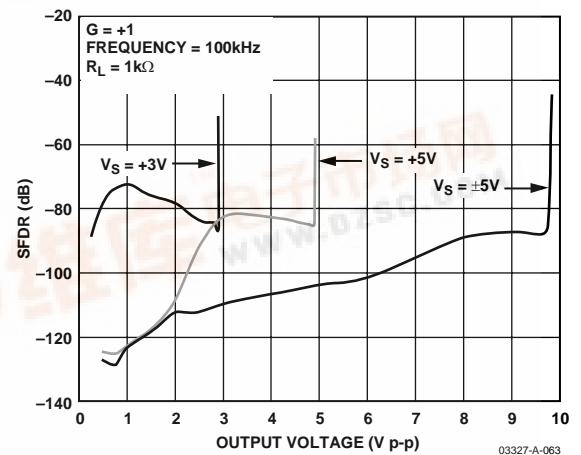
Figure 2. SFDR vs. Output Amplitude
