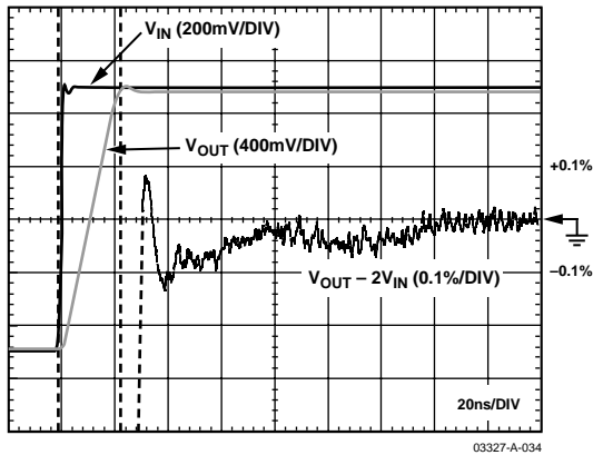
Figure 35. 0.1% Short-Term Settling Time
