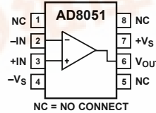
Figure 1. SOIC-8 (R)
