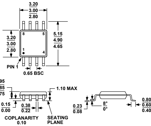
Figure 55. 8-Lead Mini Small Outline Package [MSOP] (RM-8)
