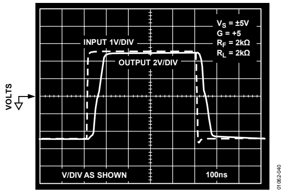
Figure 41. Overdrive Recovery
