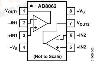
Figure 2. 8-Lead SOIC (R)/MSOP (RM)
