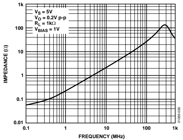
Figure 36. Output Impedance vs. Frequency, V_{\text{OUT}} = 0.2\text{V p-p} , R_L = 1\text{k}\Omega , V_S = 5\text{V}
