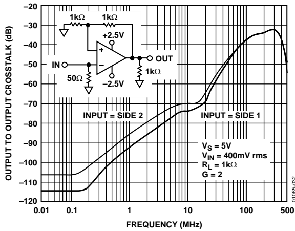
Figure 32. AD8062 Crosstalk, V_{\text{OUT}} = 2.0\text{V p-p} , R_L = 1\text{k}\Omega , G = 2 , V_S = 5\text{V}
