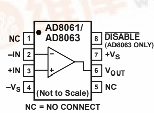
Figure 1. 8-Lead SOIC (R)
