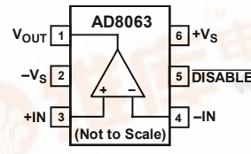
Figure 3. 6-Lead SOT-23 (RJ)
