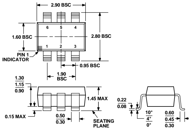
Figure 60. 6-Lead Small Outline Transistor Package [SOT-23] (RJ-6)
