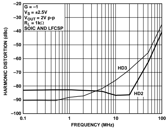
Figure 30. Harmonic Distortion vs. Frequency for Various Packages
