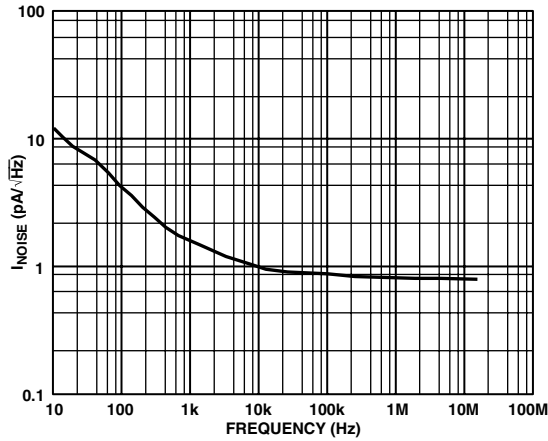
TPC 35. Current Noise vs. Frequency
