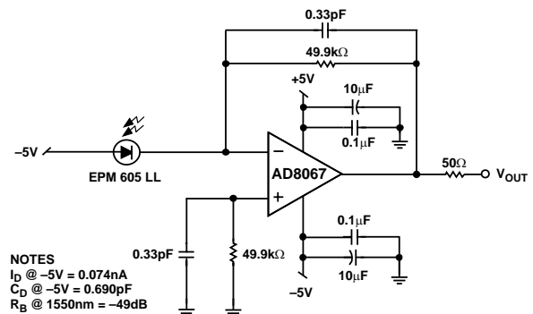
Figure 51. Photodiode Preamplifier
