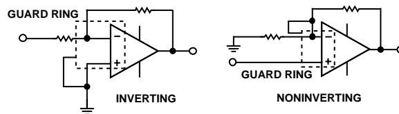
Figure 47. Guard-Ring Configurations
