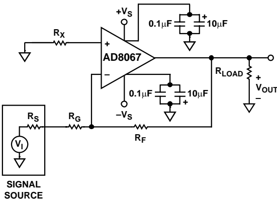
Figure 42. Inverting Gain Configuration
