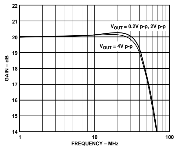
Figure 9. Frequency Response for Various Output Amplitudes
