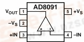
Figure 2. SOT23-5 (RT-5)
