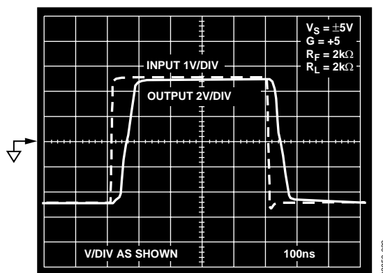
Figure 32. Overdrive Recovery
