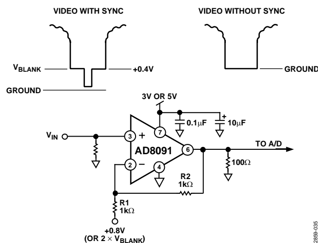
Figure 35. Sync Stripper
