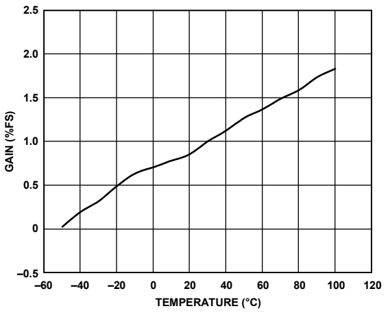
Figure 13. Gain vs. Temperature
