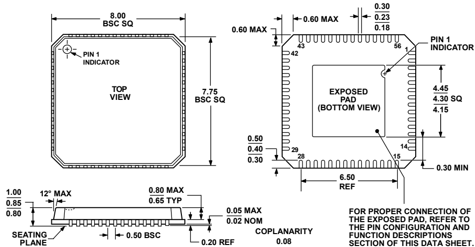
Figure 34. 56-Lead Lead Frame Chip Scale Package [LFCSQ_VQ] 8 mm × 8 mm Body, Very Thin Quad (CP-56-2) Dimensions shown in millimeters
