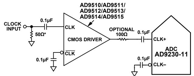
Figure 28. Single-Ended 3.3 V CMOS Sample Clock
