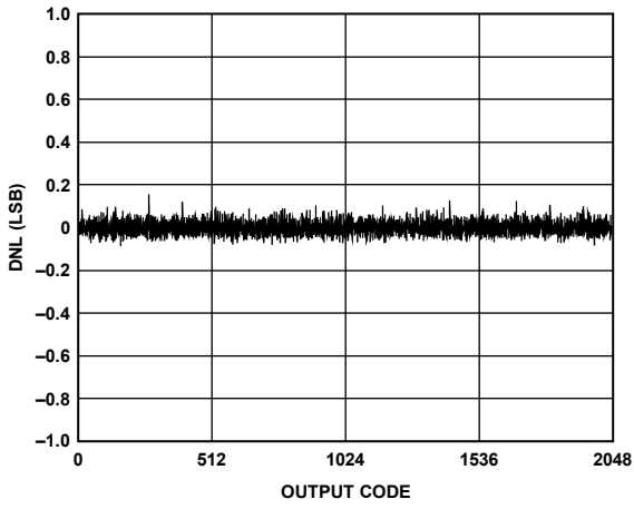
Figure 12. DNL
