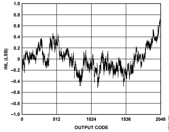
Figure 14. INL
