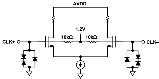
Figure 15. Clock Inputs
