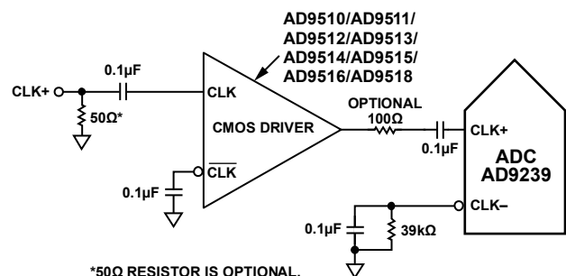
Figure 55. Single-Ended 1.8 V CMOS Sample Clock
