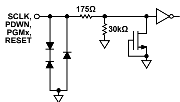
Figure 37. Equivalent SCLK, PDWN, PGMx, RESET Input Circuit
