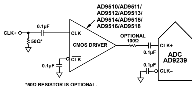
Figure 56. Single-Ended 3.3 V CMOS Sample Clock
