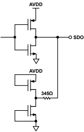
Figure 44. Equivalent SDO Output Circuit
