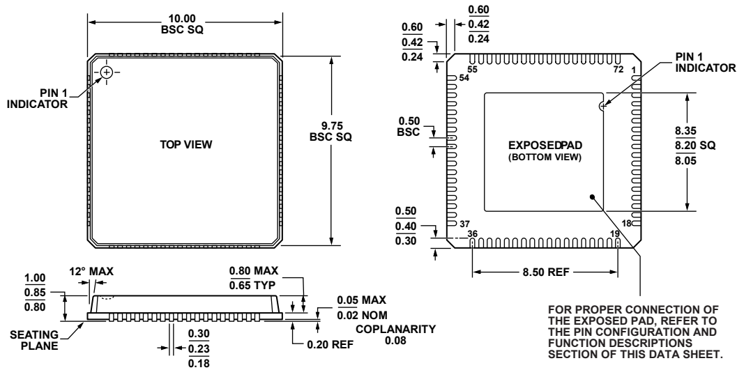
Figure 80. 72-Lead Lead Frame Chip Scale Package [LFCSP_VQ] 10 mm x 10 mm Body, Very Thin Quad (CP-72-3)
