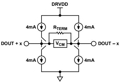
Figure 43. Equivalent Digital Output Circuit
