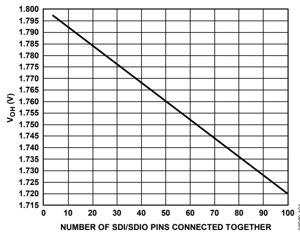
Figure 77. SDI/SDIO Pin Loading
