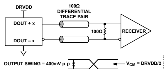
Figure 61. DC-Coupled Digital Output Termination Example
