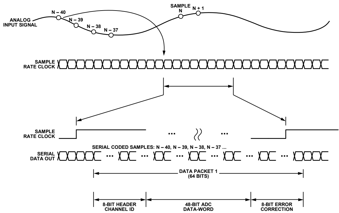
Figure 2. Timing Diagram
