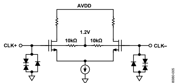
Figure 35. CLK± Inputs
