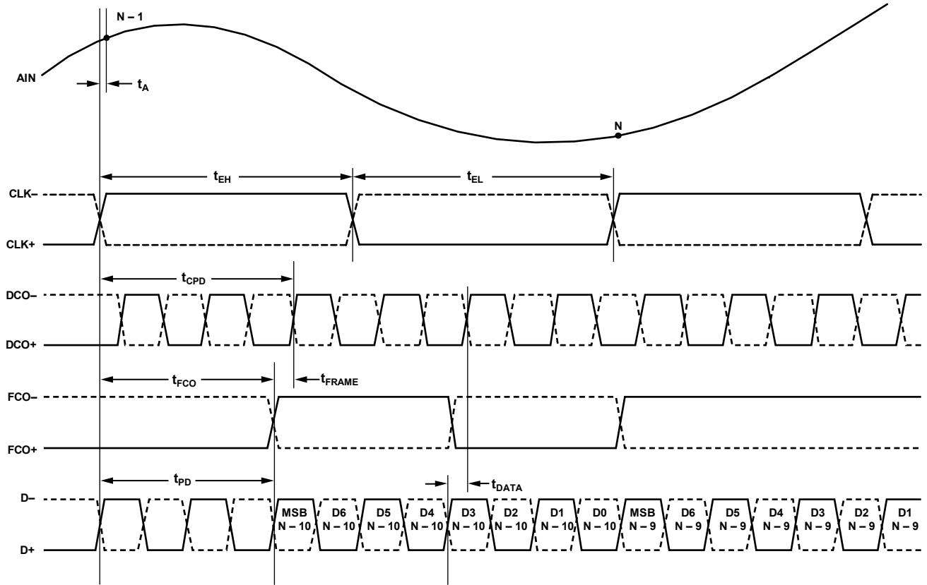
Figure 2. 8-Bit Data Serial Stream (Default)
