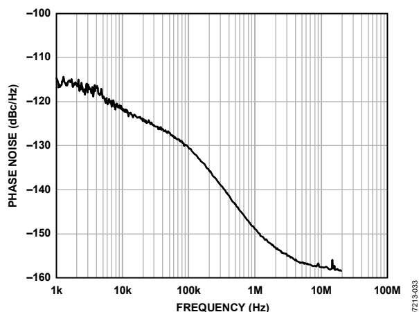
Figure 31. Phase Noise (Absolute) Clock Generation; Internal VCO @ 2.703 GHz; PFD = 15.36 MHz; LBW = 63 kHz; LVPECL Output = 122.88 MHz
