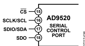
Figure 59. Serial Control Port
