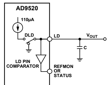
Figure 42. Current Source Lock Detect
