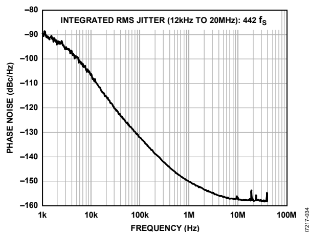
Figure 32. Phase Noise (Absolute) Clock Cleanup; Internal VCO @ 1.552 GHz; PFD = 19.44 MHz; LBW = 1.84 kHz; LVPECL Output = 155.52 MHz
