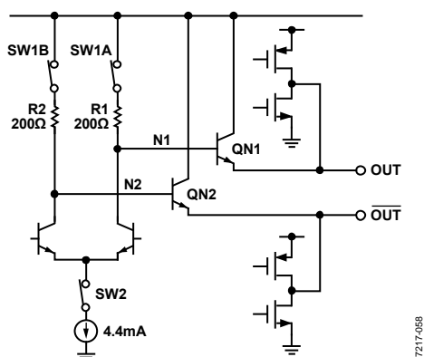
Figure 51. LVPECL Output Simplified Equivalent Circuit
