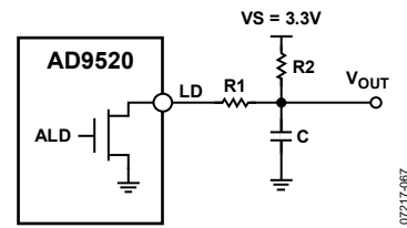
Figure 41. Example of Analog Lock Detect Filter, Using N-Channel Open-Drain Driver
