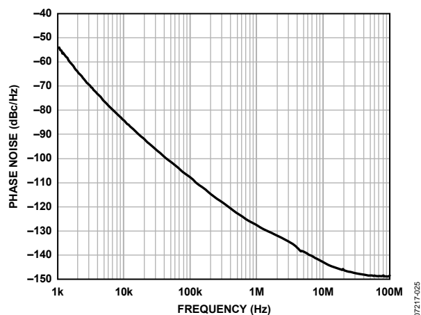
Figure 25. Internal VCO Phase Noise (Absolute) Direct-to-LVPECL @ 1800 MHz
