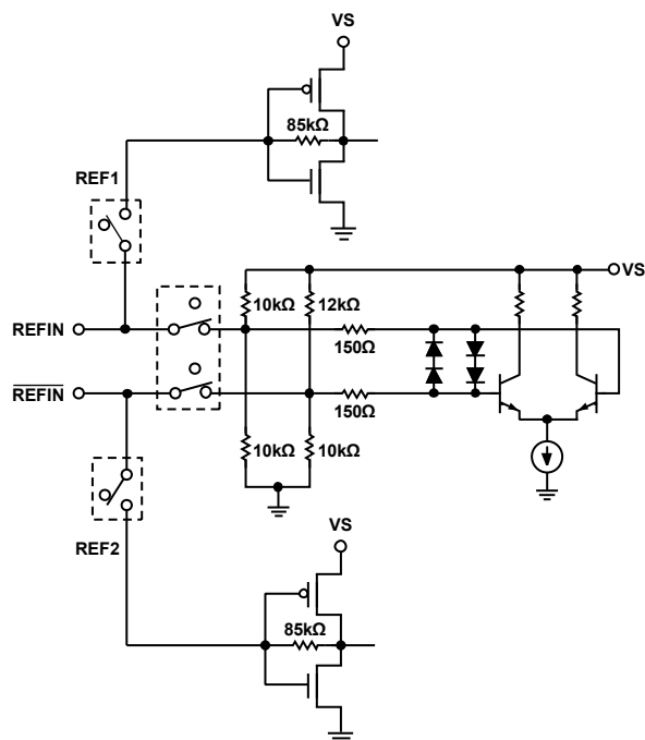
Figure 40. REF IN Equivalent Circuit for NonXTAL Mode
