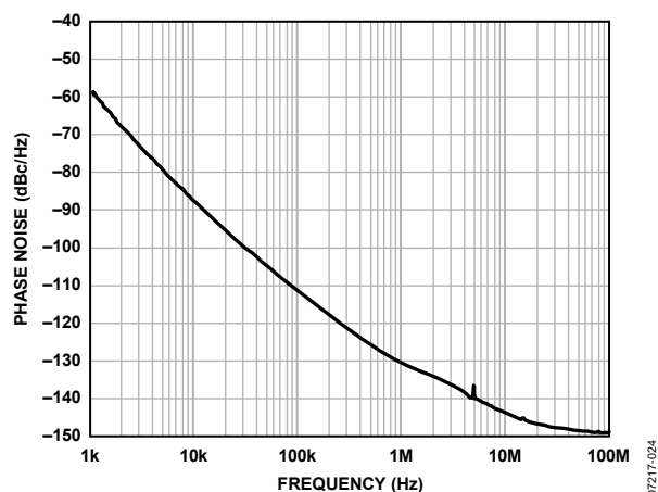
Figure 24. Internal VCO Phase Noise (Absolute) Direct-to-LVPECL @ 1625 MHz
