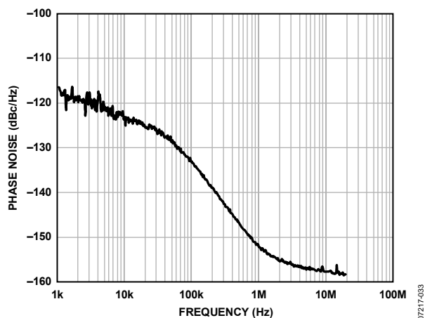
Figure 31. Phase Noise (Absolute) Clock Generation; Internal VCO @ 1.475 GHz; PFD = 15.36 MHz; LBW = 40 kHz; LVPECL Output = 122.88 MHz
