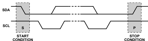
Figure 44. Start and Stop Conditions
