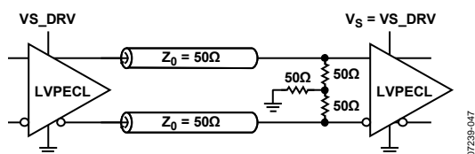
Figure 59. DC-Coupled 3.3 V LVPECL Y-Termination
