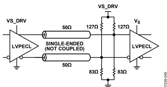
Figure 58. DC-Coupled 3.3 V LVPECL Far-End Thevenin Termination
