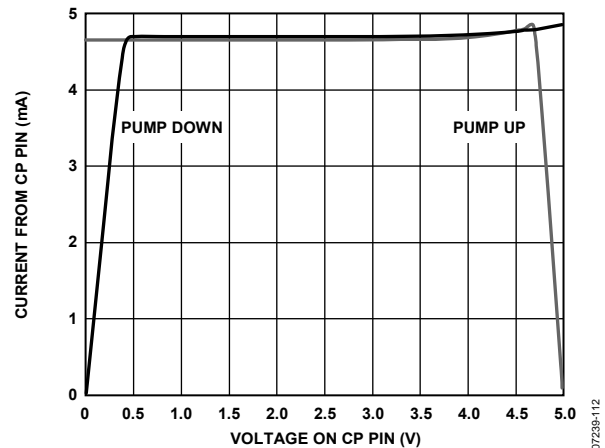
Figure 9. Charge Pump Characteristics @ V_{CP} = 5.0 V
