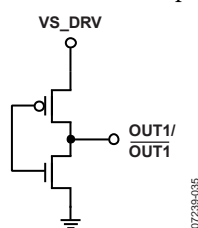
Figure 42. CMOS Equivalent Output Circuit
