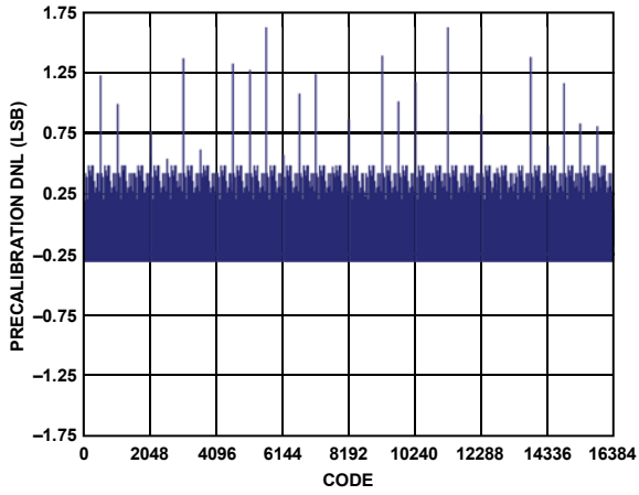
Figure 12. AD9717 Precalibration DNL at 3.3 V
