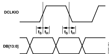
Figure 81. Set-Up and Hold Times for All Input Modes
