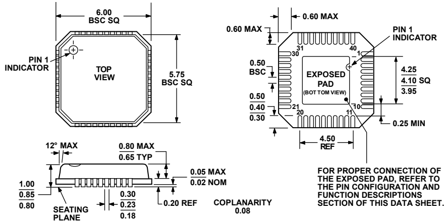
Figure 98. 40-Lead Lead Frame Chip Scale Package [LFCSP_VQ] 6 mm × 6 mm, Very Thin Quad (CP-40-1) Dimensions shown in millimeters
