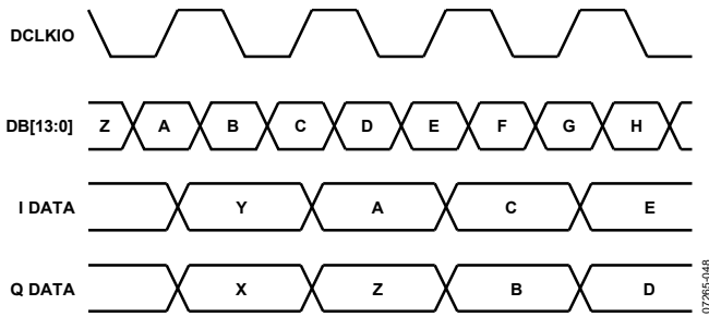
Figure 78. Timing Diagram with IFIRST = 0, IRISING = 1
