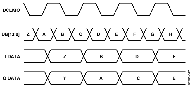
Figure 77. Timing Diagram with IFIRST = 0, IRISING = 0
