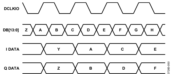
Figure 80. Timing Diagram with IFIRST = 1, IRISING = 1
