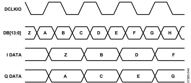
Figure 79. Timing Diagram with IFIRST = 1, IRISING = 0
