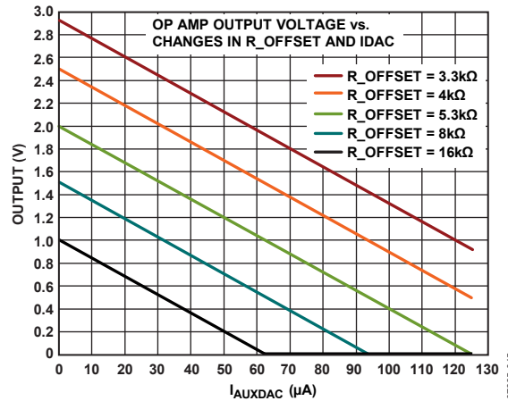
Figure 93. AUXDAC Op Amp Output vs. Current, AVDD = 3.3 \text{ V} No Load, AUXDAC 0x1FF to 0x000
