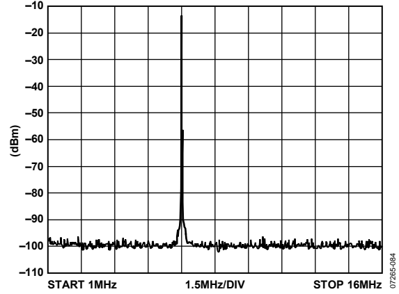
Figure 63. AD9717 Single Tone 1.8 V
