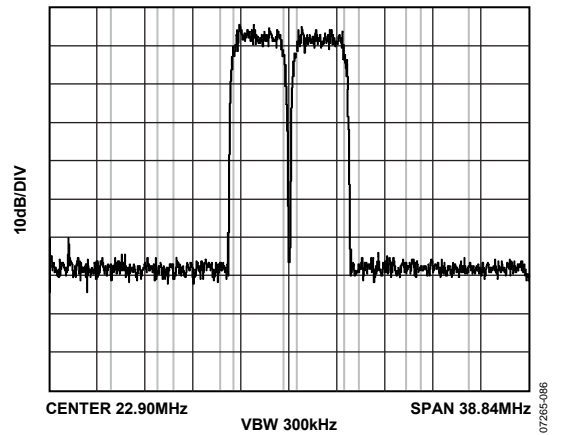
Figure 65. AD9717 ACLR 2-Carrier 3.3 V
