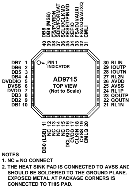
Figure 4. AD9715 Pin Configuration
