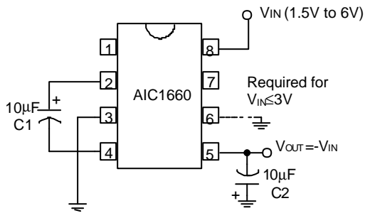
Fig. 8 Negative Voltage Converter
