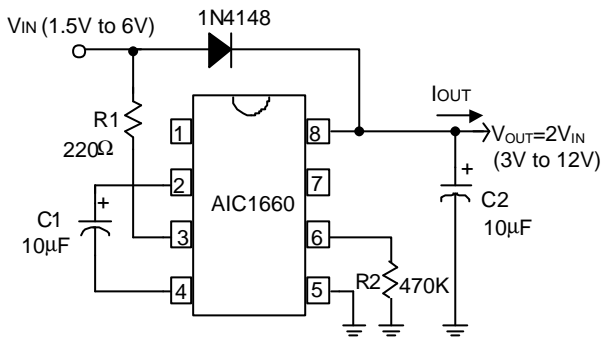
Fig. 9 Voltage Doubling
