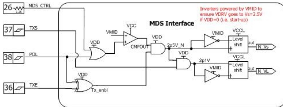
Figure 8: MDS Interface
