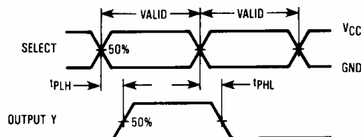
Figure 2. Switching Waveforms
