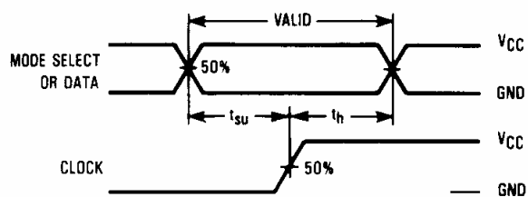
Figure 4. Switching Waveforms
