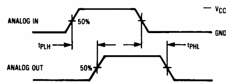
Figure 3. Switching Waveforms
