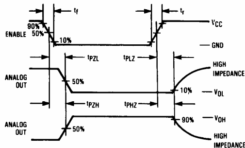
Figure 5. Switching Waveforms
