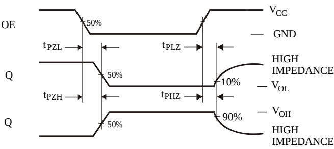
Figure 2. Switching Waveforms
