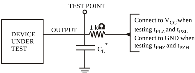
Figure 5. Test Circuit
