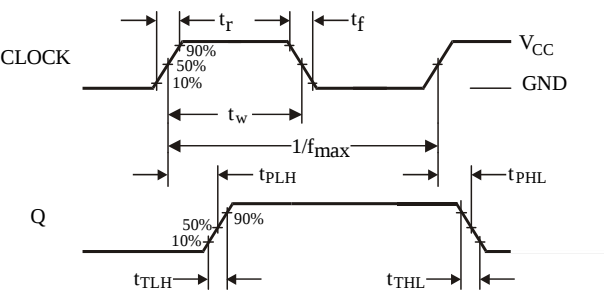
Figure 1. Switching Waveforms
