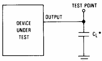
Figure 9. Test Circuit
