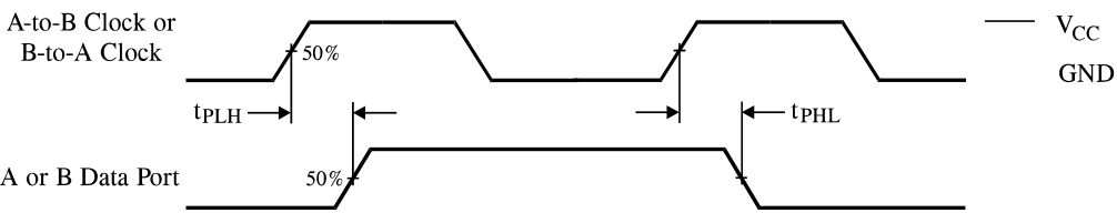
Figure 1. Switching Waveforms
