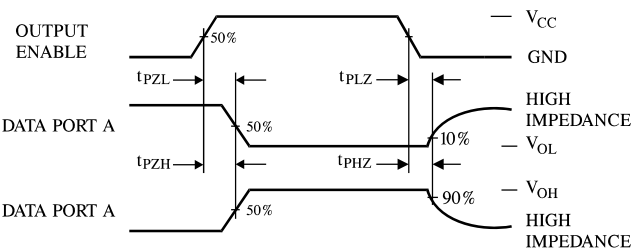
Figure 5. Switching Waveforms
