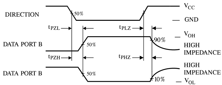
Figure 6. Switching Waveforms
