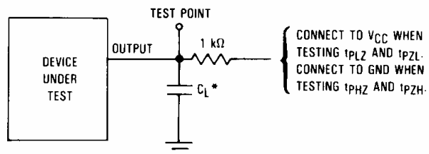
Figure 10. Test Circuit
